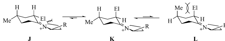
Figure 4. Conformational preference for product formation.
