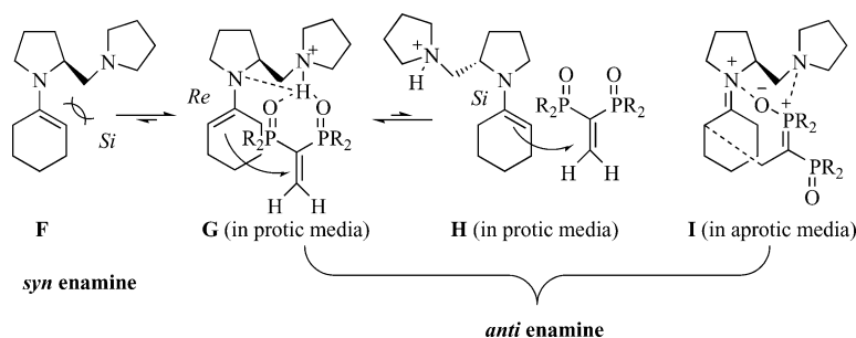
Figure 3. Proposed facial selectivity for the transition state.
